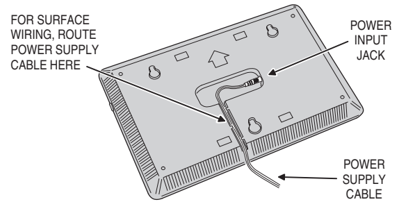
Figure 2 SP2 Touch Screen Power Input Connector
