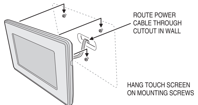
Figure 3 SP2 Touch Screen Recessed Power Wiring
